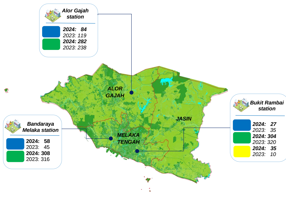
Exhibit 1.4: Status of air quality by station, Melaka, 2023 and 2024
