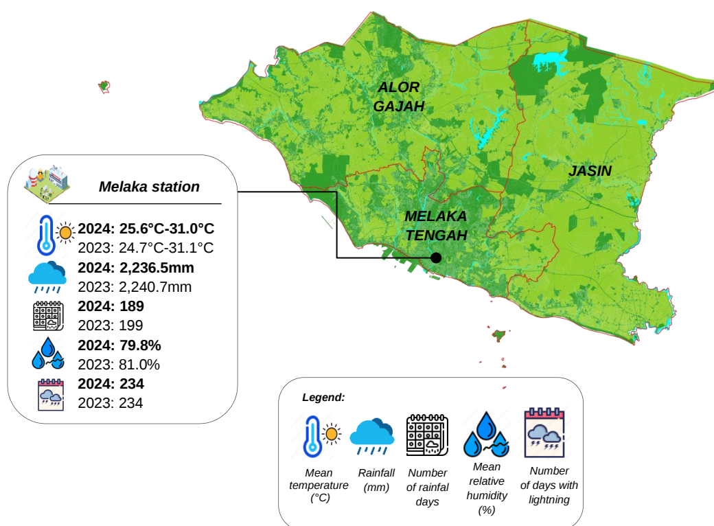
Exhibit 1.3: Summary of climate statistics at meteorological stations, Melaka, 2023 and 2024
