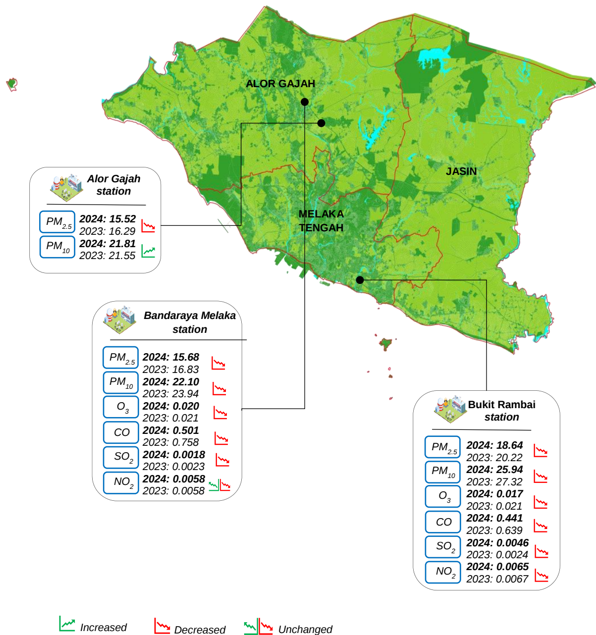
Exhibit 1.2: Summary of air pollutants statistics by station, Melaka, 2023 and 2024
