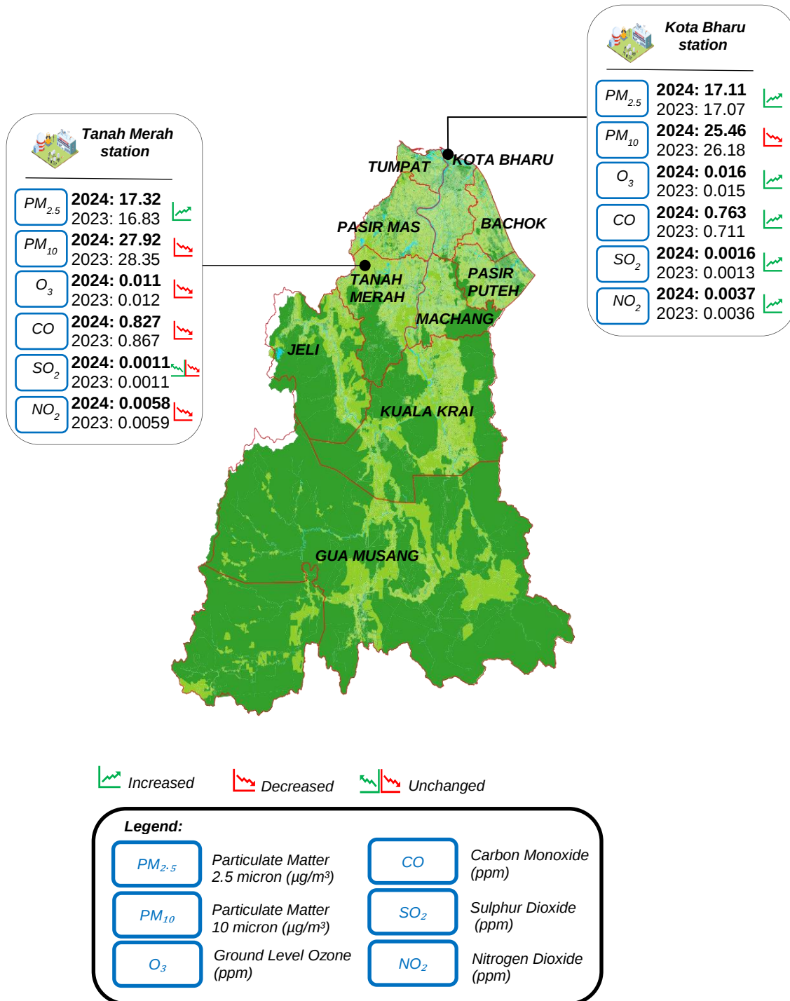
Exhibit 1.2: Summary of air pollutants statistics by station, Kelantan, 2023 and 2024
