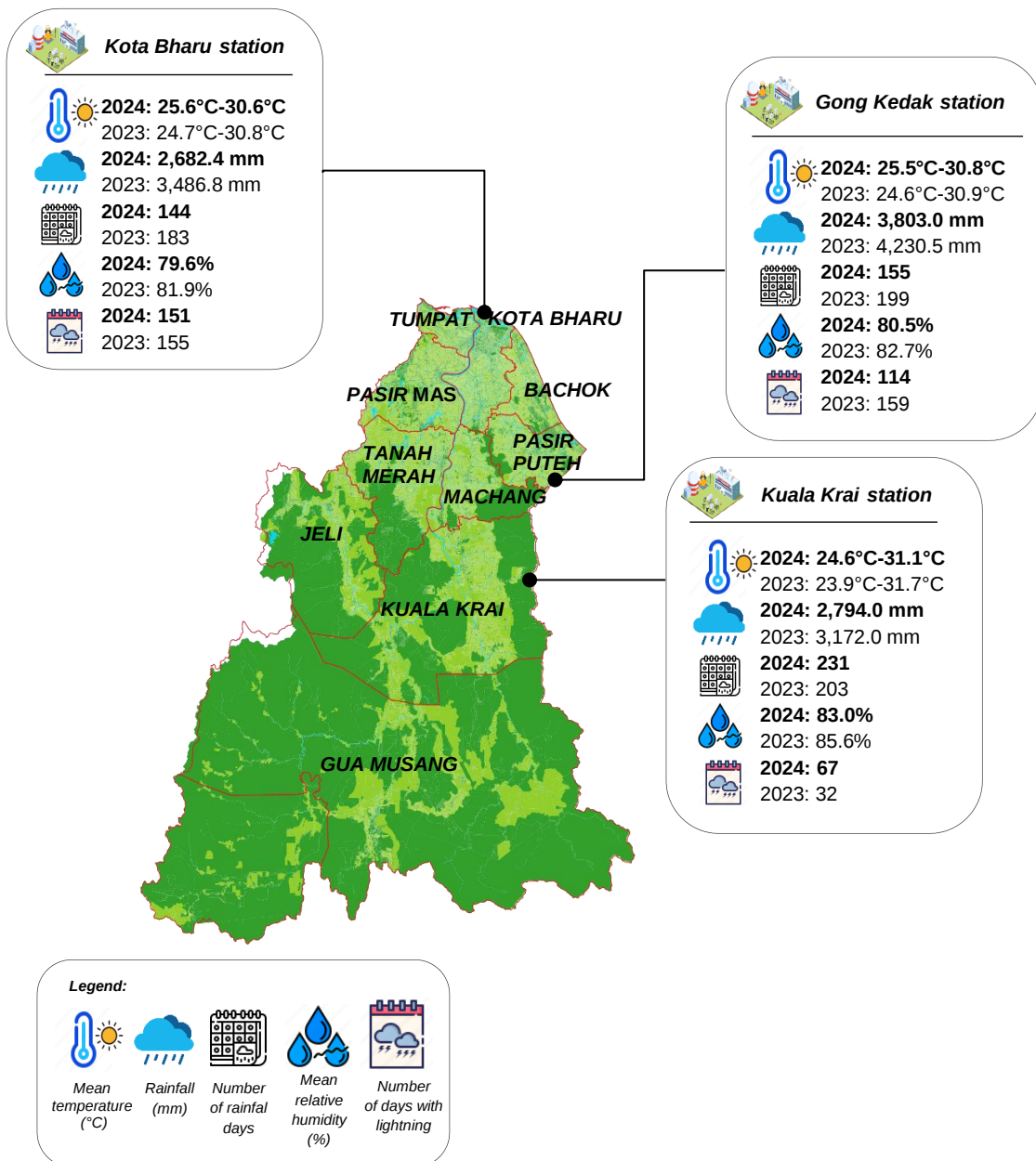
Exhibit 1.3: Summary of climate statistics at meteorological stations, Kelantan, 2023 and 2024
