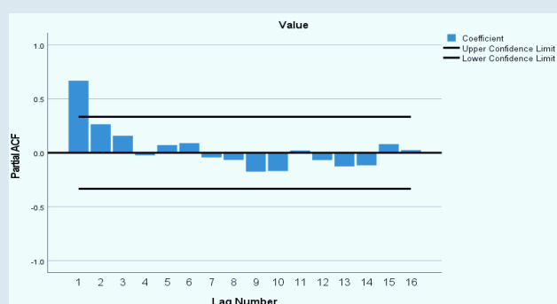
Chart 1c: PACF Plot before differencing
