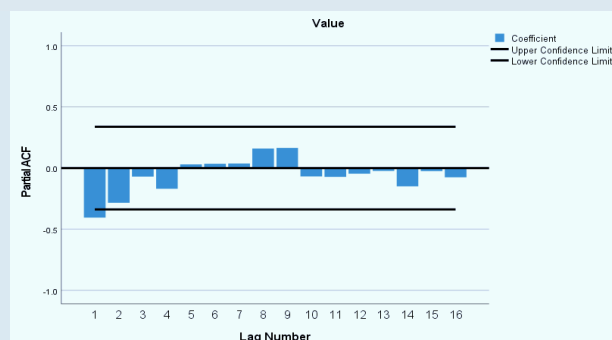
Chart 1e: PACF Plot after differencing, d=1
