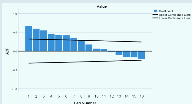
Chart 1b: ACF Plot before differencing
