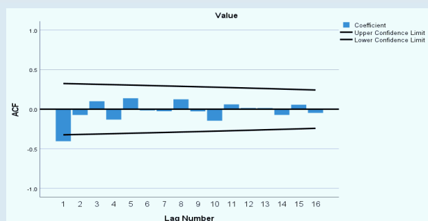
Chart 1d: ACF Plot after differencing, d=1
